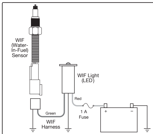
Figure 3 - WIF Wiring
