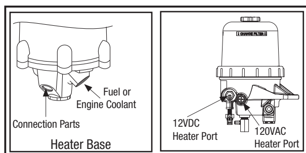
Figure 4 - Heater Base
