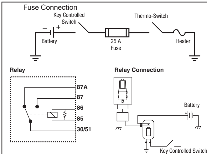
Figure 5 - Fuse and Relay Connects
